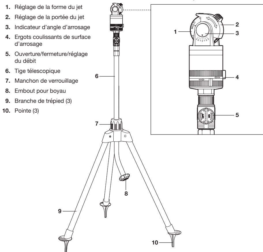
Sprinkler Head
