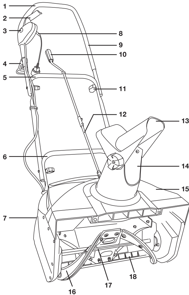
Figure 1-1 (Model SJ620-RM)
